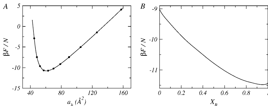
FIGURE 2 (A) Free energy per molecule as a function of the area per lipid headgroup, a_h , for a mixed lipid layer with n_L = 14 and X_B = 0.50 . (B) The optimal free energy per molecule as a function of the layer bolalipid concentration, X_B , for a mixed lipid layer with n_L = 14 . The optimal free energy is obtained from the minimum of a curve (as shown in A) for each composition.
